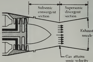
FIGURE 2-35. Convergent-divergent exhaust duct (nozzle).
